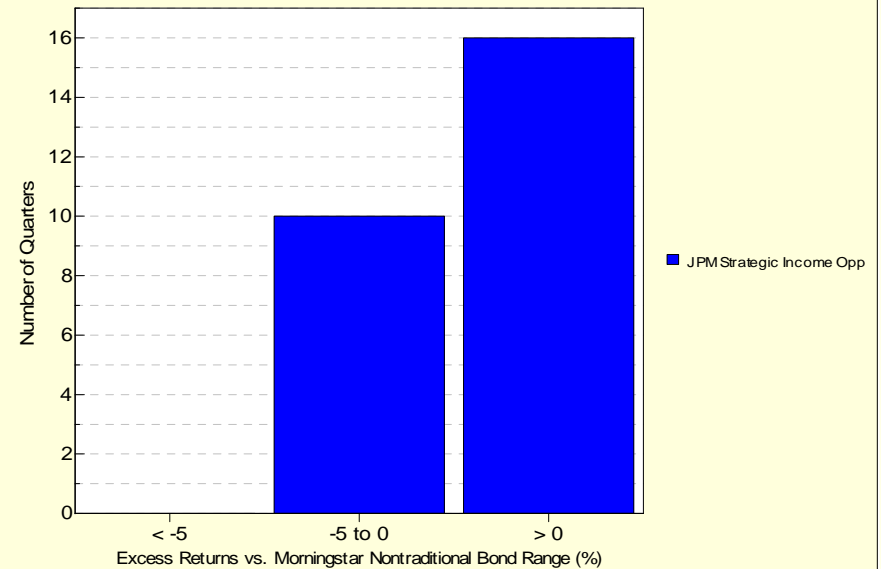
Histogram of Excess Returns vs. Morningstar Nontraditional Bond January 2009 - June 2015
