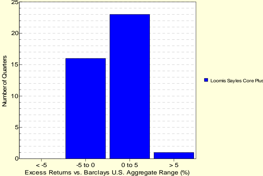
Histogram of Excess Returns vs. Barclays U.S. Aggregate July 2005 - June 2015
