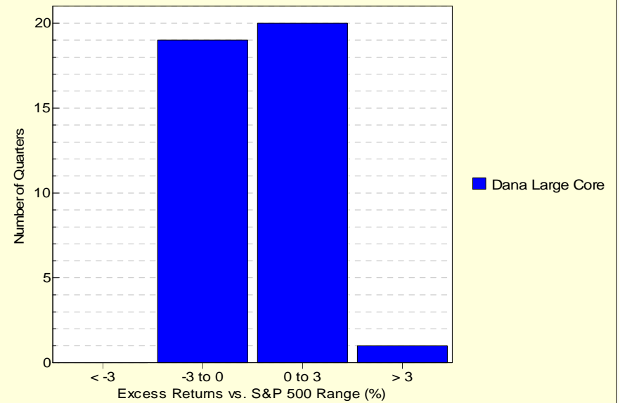
Histogram of Excess Returns vs. S&P 500 July 2005 - June 2015
