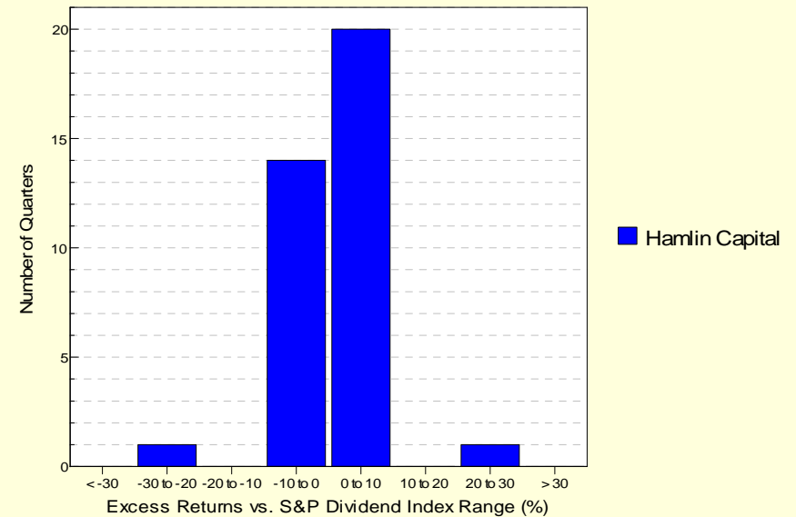
Histogram of Excess Returns vs. S&P Dividend Index July 2006 - June 2015
