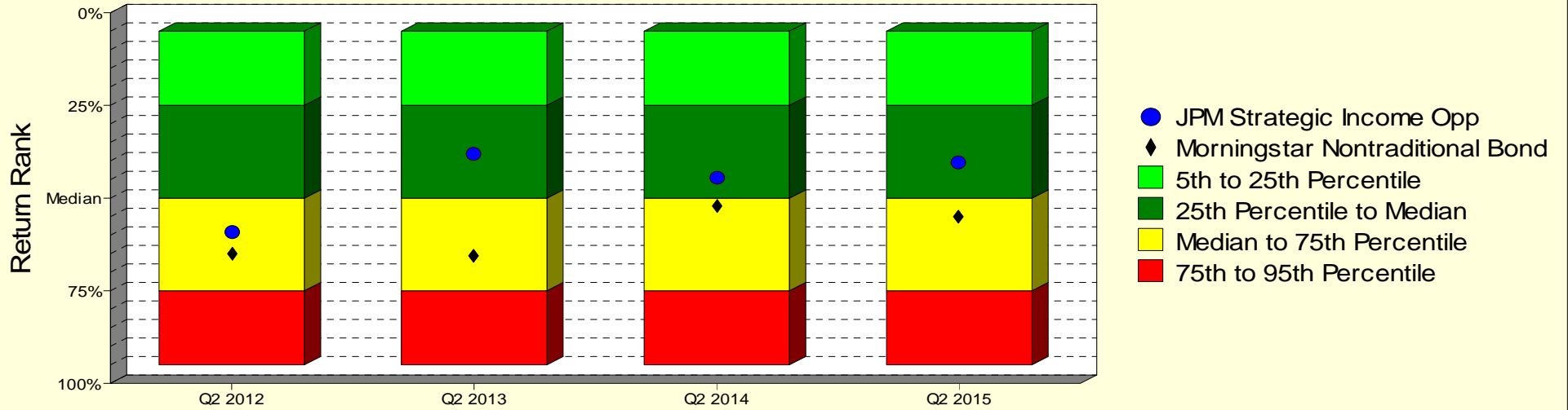
Manager vs Universe: Return Rank 12-Quarter Moving Windows, Computed Yearly
