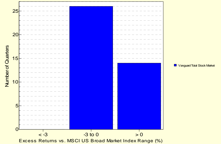
Histogram of Excess Returns v.s. MSCI US Broad Market Index July 2005 - June 2015
