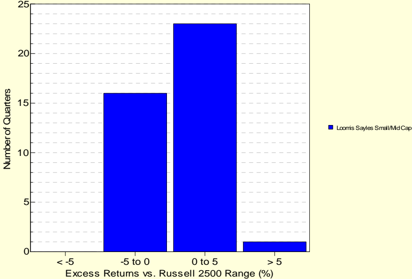
Histogram of Excess Returns vs. Russell 2500 July 2005 - June 2015
