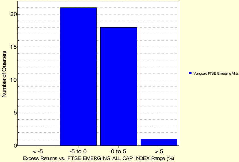
Histogram of Excess Returns vs. FTSE EMERGING ALL CAP INDEX July 2005 - June 2015
