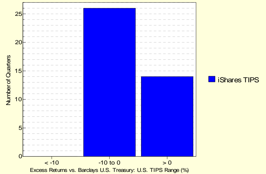
Histogram of Excess Returns vs. Barclays U.S. Treasury: U.S. TIPS July 2005 - June 2015
