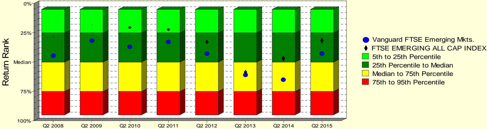
Manager vs Universe: Return Rank 12-Quarter Moving Windows, Computed Yearly
